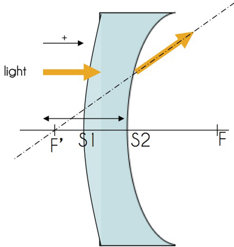
Meniscus lens (-) : diverging lens Used to correct myopia
